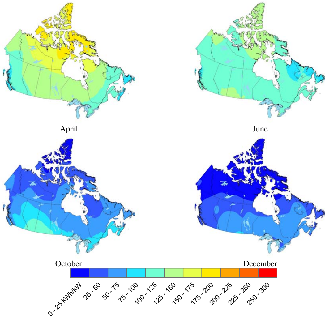
Figures 4-7: Monthly PV potential maps at latitude tilt for April, June, October and December.
